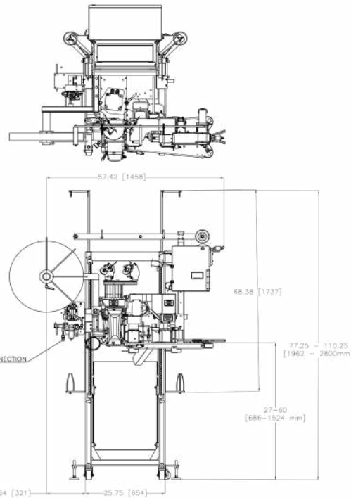
LAYOUT FOR 501T SEWING SYSTEM REVISION 1 32" INFEED 4/22/2020
